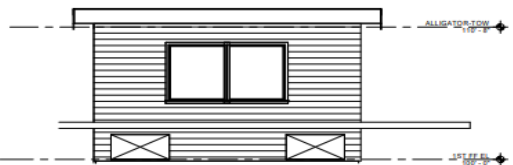
(D1) Alligator North 3/4" = 1'-0"
