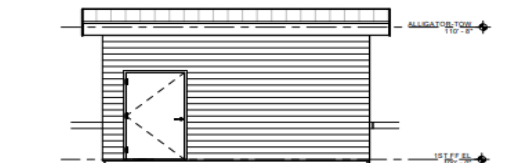
(B1) Alligator South 3/4" = 1'-0"
